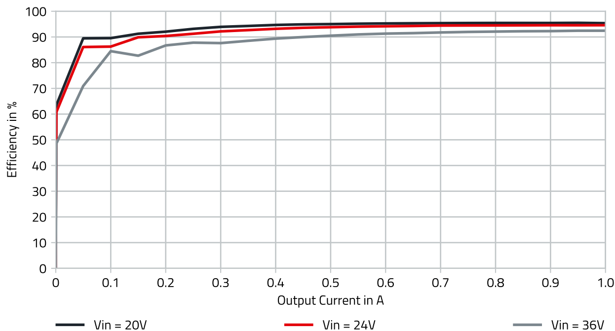
Figure 4: Efficiency.
