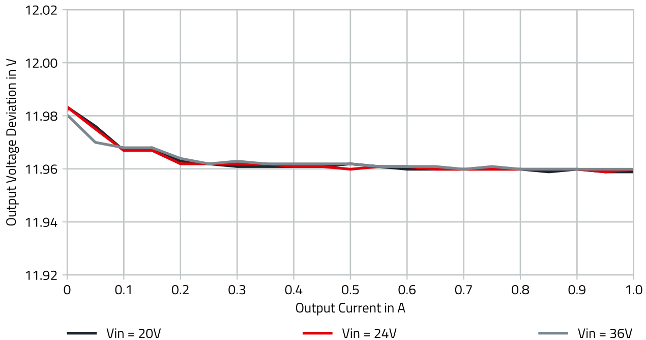
Figure 6: Load regulation.
