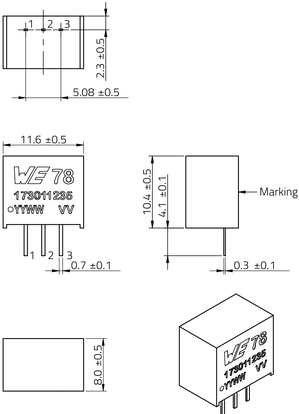
Figure 18: Physical dimensions.
