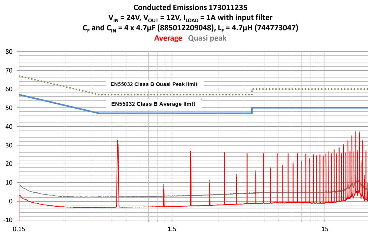
Figure 3: Conducted EMI with input filter.
