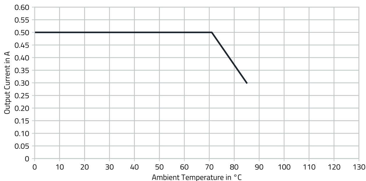
Figure 5: Thermal derating.
