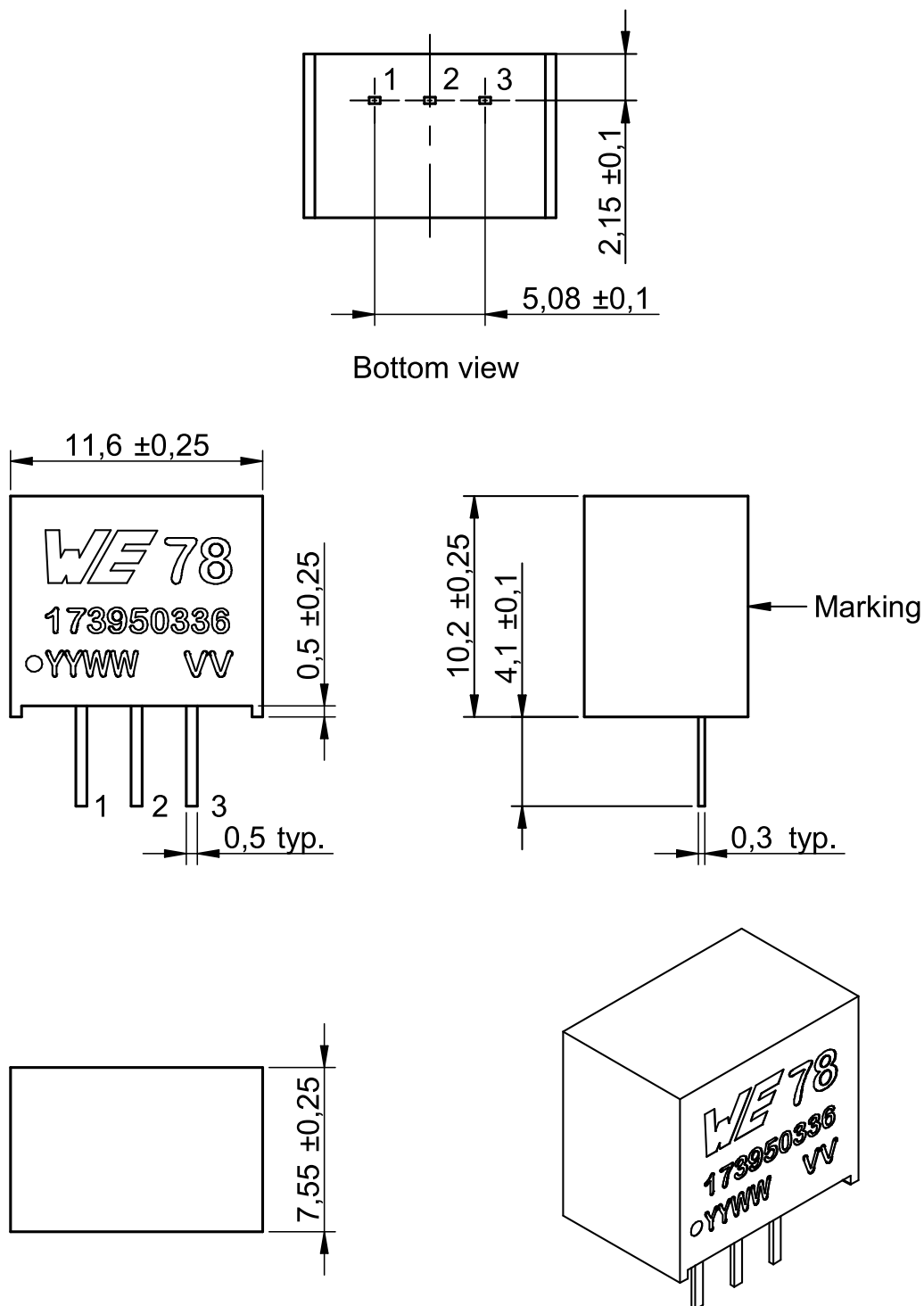
Figure 16: Physical dimensions.
