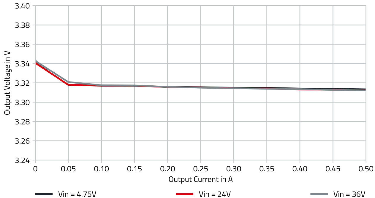
Figure 6: Load regulation.
