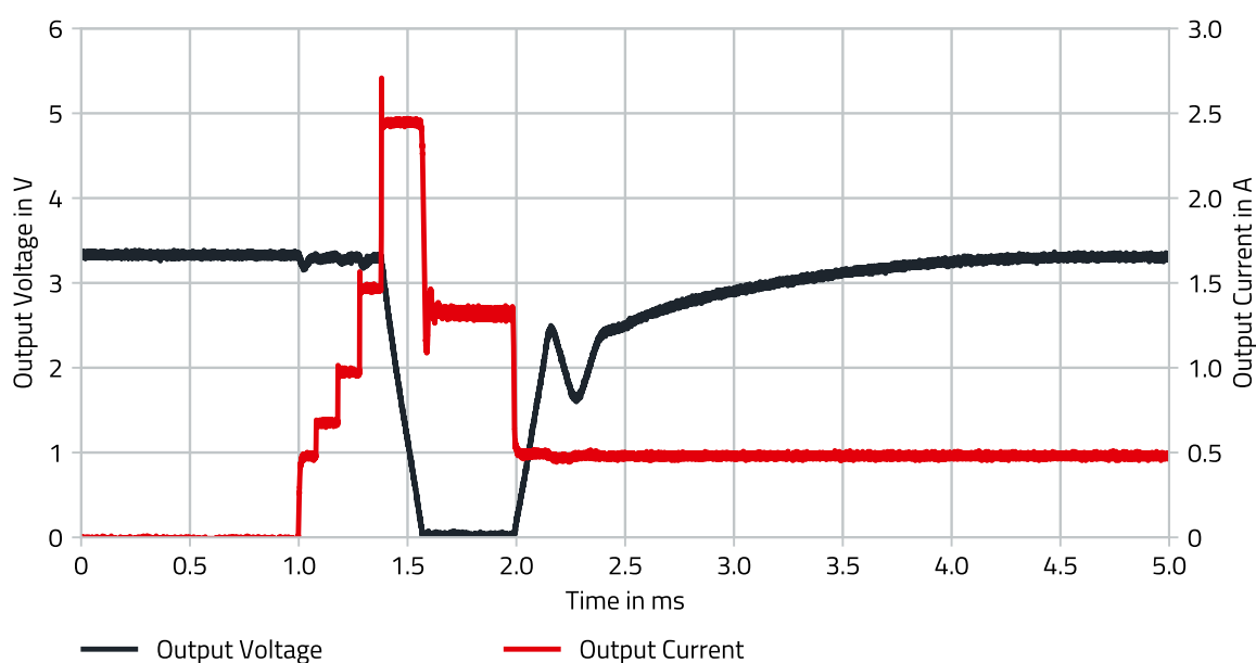
Figure 12: Over current protection.
