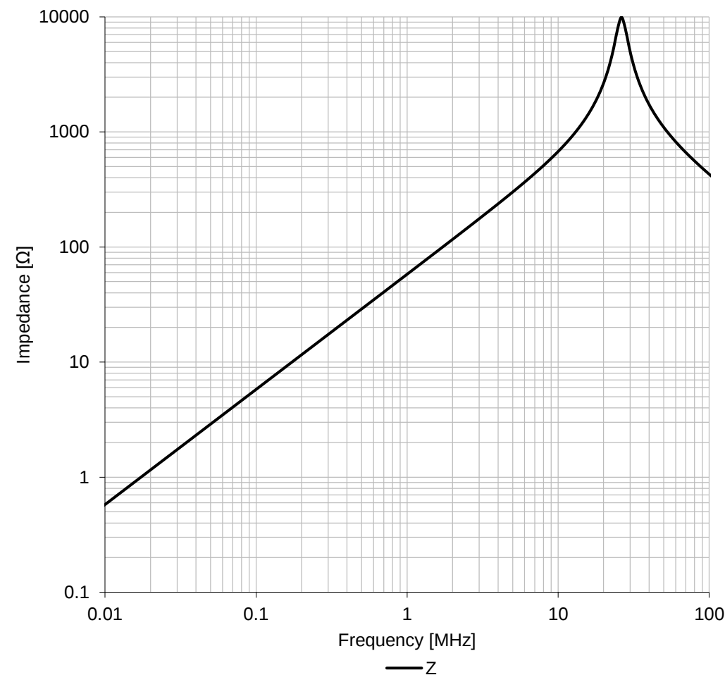
Typical Impedance Characteristics:
