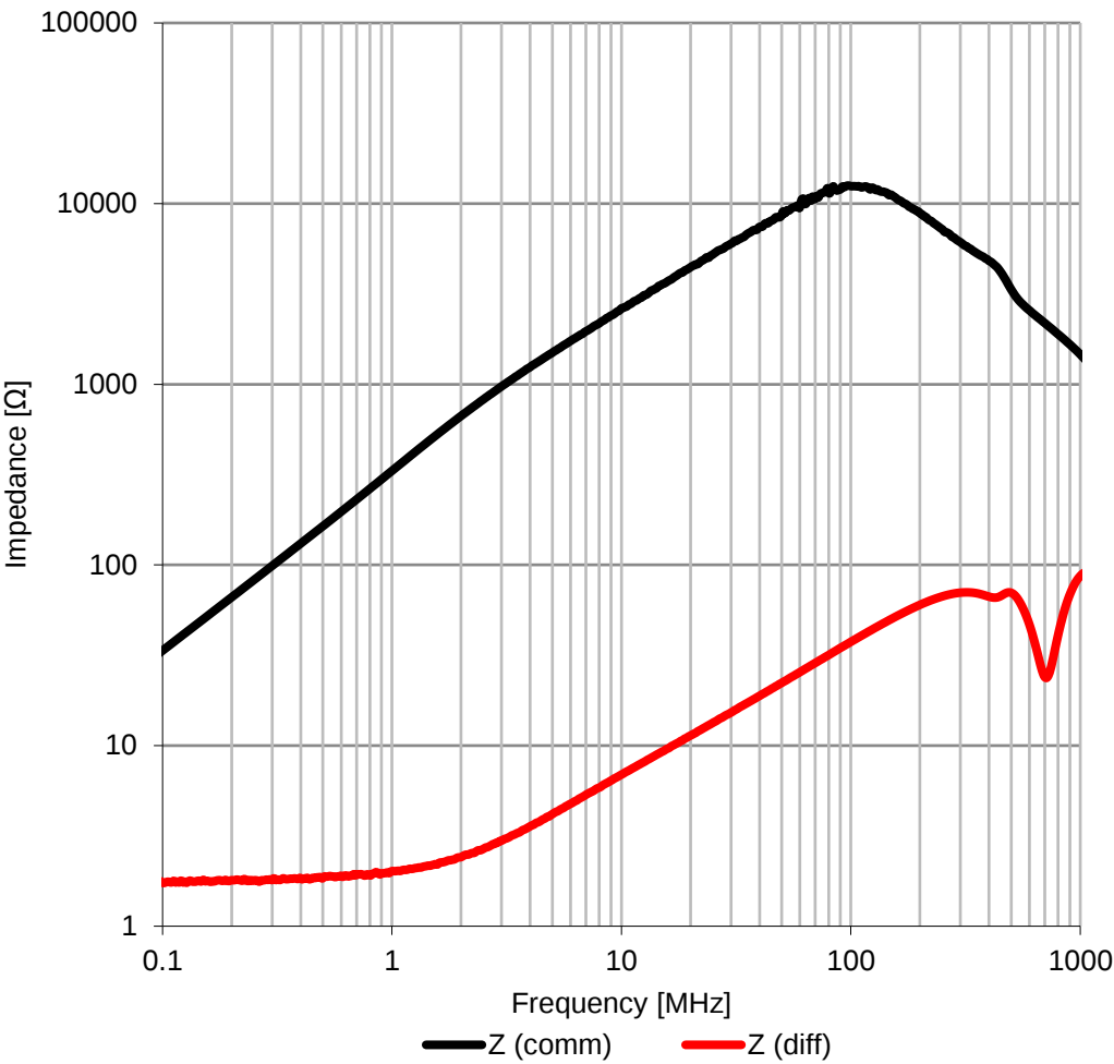
Typical Impedance vs. Frequency:
