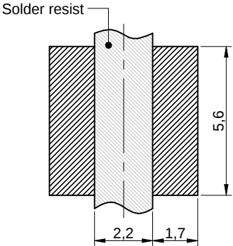
No vias and traces underneath the inductor Scale - 5:1
