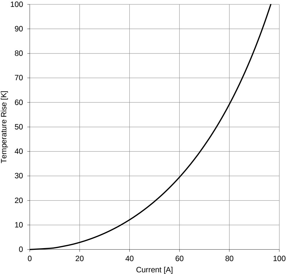
Typical Temperature Rise vs. Current Characteristics - One Turn:
